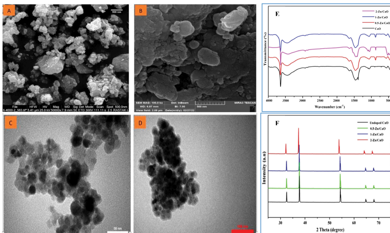
Fig 4 | (a) FE-SEM images of \text{Fe}_3\text{O}_4 , 41 (b) FE-SEM images of the as-prepared nanocatalyst, 41 (c) TEM images of \text{Fe}_3\text{O}_4 , 41 (d) TEM images of the as-prepared nanocatalyst, 41 (e) FT-IR spectra of undoped and Zn-doped CaO nanocatalysts, 41 and (f) XRD patterns of undoped and Zn-doped CaO nanocatalysts 41
